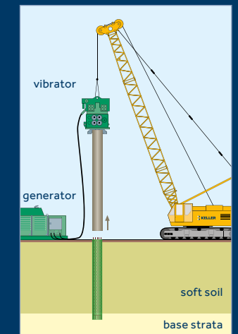
Withdrawal of casing by drilling rig or alternatively using vibrator
