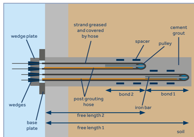
Pre-stressed removable strand anchors
