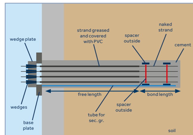
Pre-stressed temporary anchors
