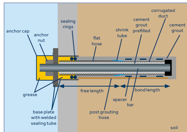
Pre-stressed permanent bar anchors (simplified)
