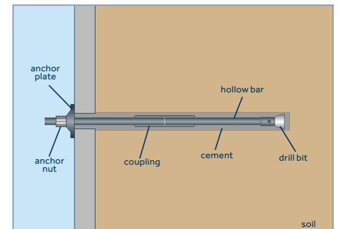
Soil nail with hollow bar
