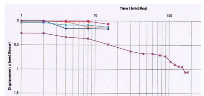
Suitability test: Determination of creep values
