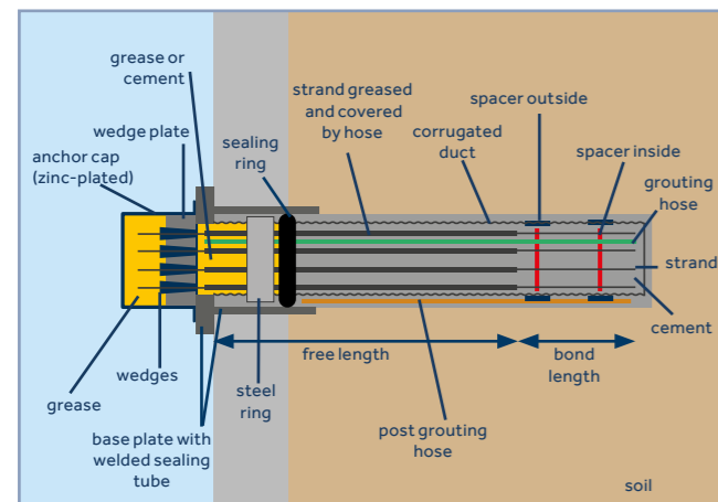
Pre-stressed permanent strand anchors (simplified)
